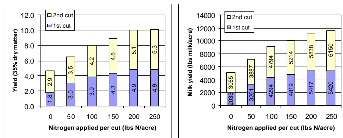
Figure 2: Brown mid rib sorghum sudangrass dry matter yield (left) and milk yield per acre (right) as affected by the amount of nitrogen applied at the Mt Pleasant Research Farm, NY, in 2002.
